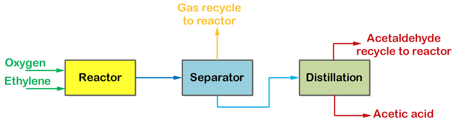
Figure: Manufacture of acetic acid by ethylene oxidation
